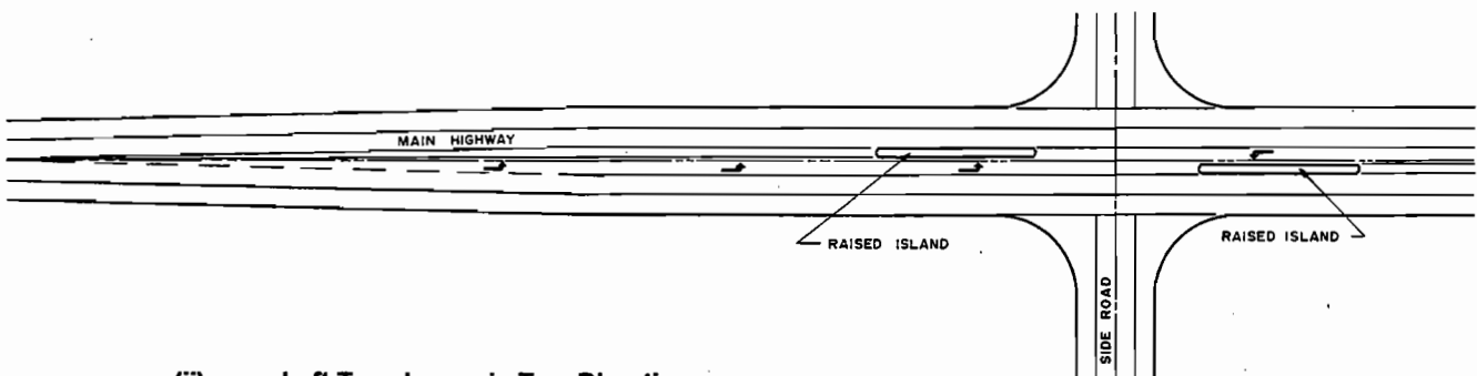
Figure E10-4 Offset Divisional Islands at 'Cross' Intersections
