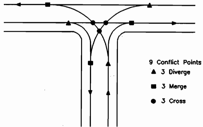
T-INTERSECTION
