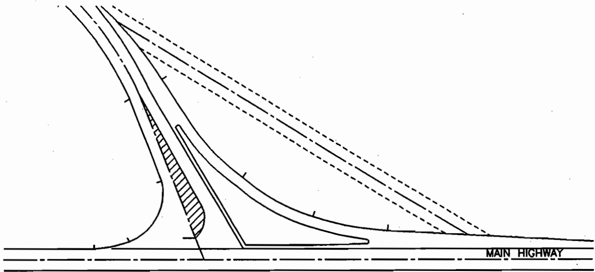
PREFERRED DESIGN
